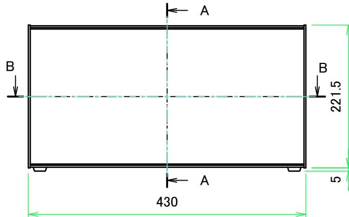
A view
